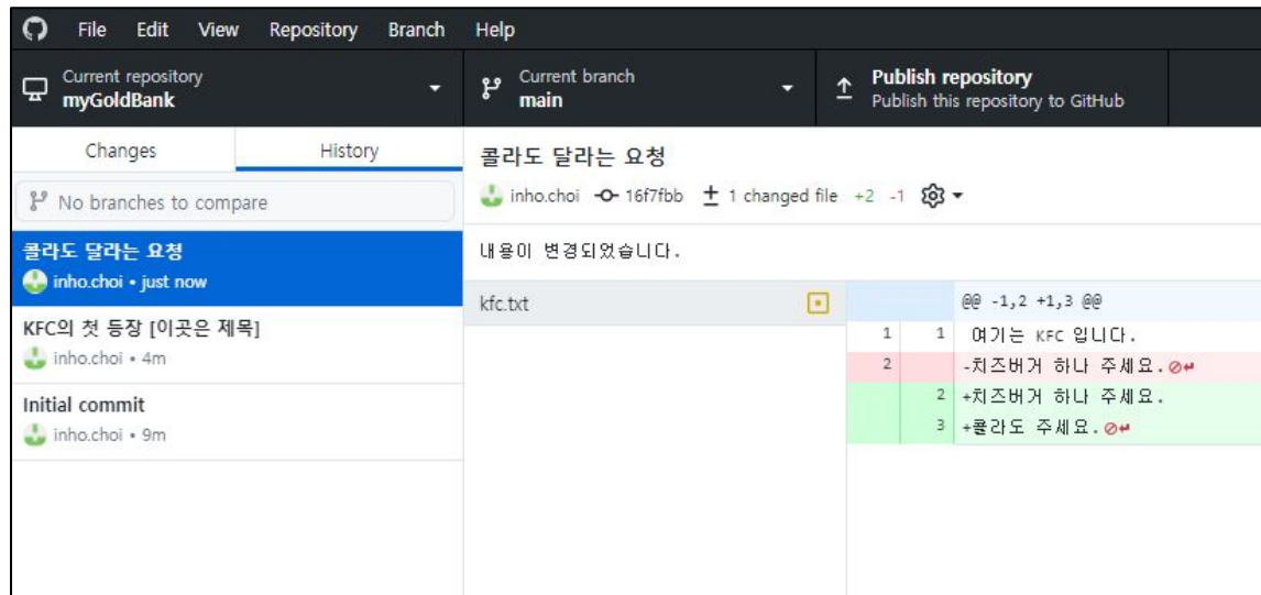
Github Desktop
