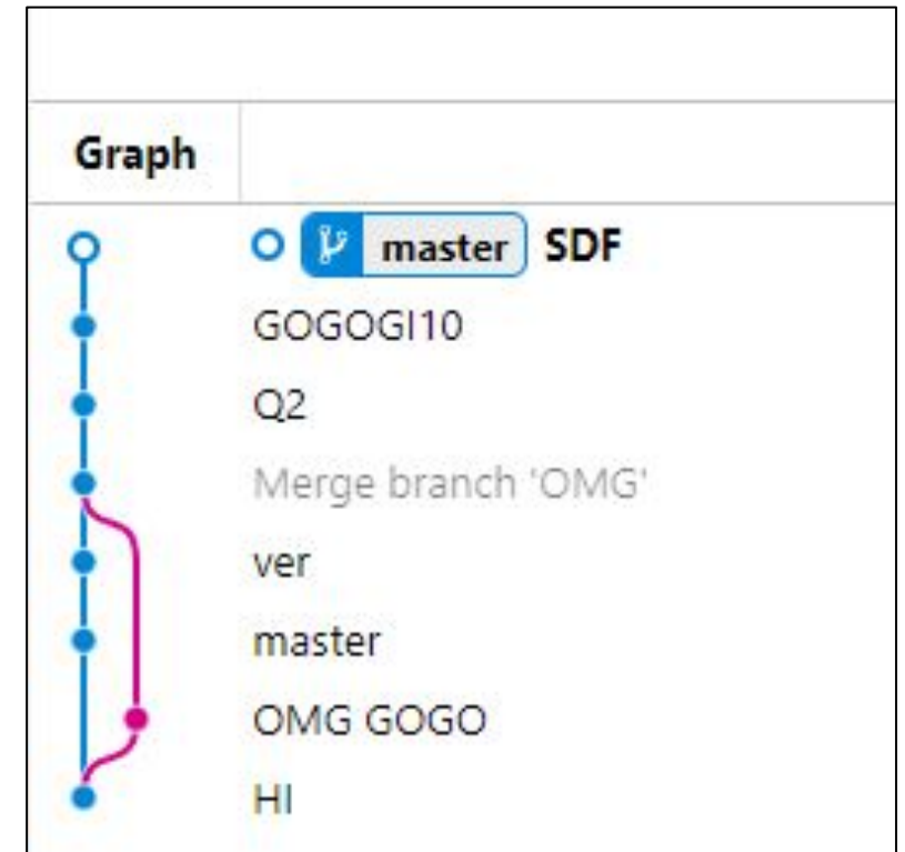
VSCode Plugin
